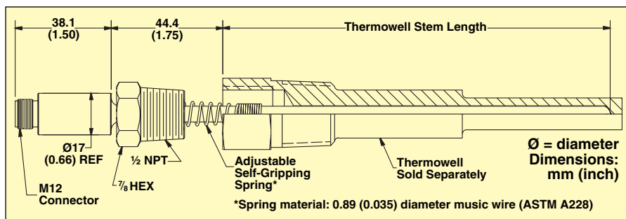
M12C-SIL-K-R-F-1.5 mating cable sold separately. Visit omega.com/m12c for optional extension cables.
